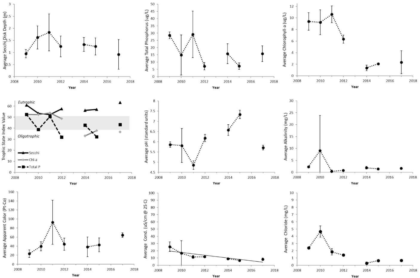
Annual average values of select water quality indicators for Otter Pond 2009-2017. Vertical bars represent ± 1 standard deviation of the mean; Solid trend lines across the data indicate a statistically significant trend ( p < 0.05 ).
